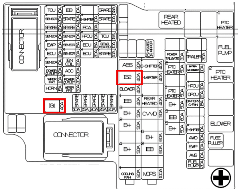
Engine compartment fuse box
