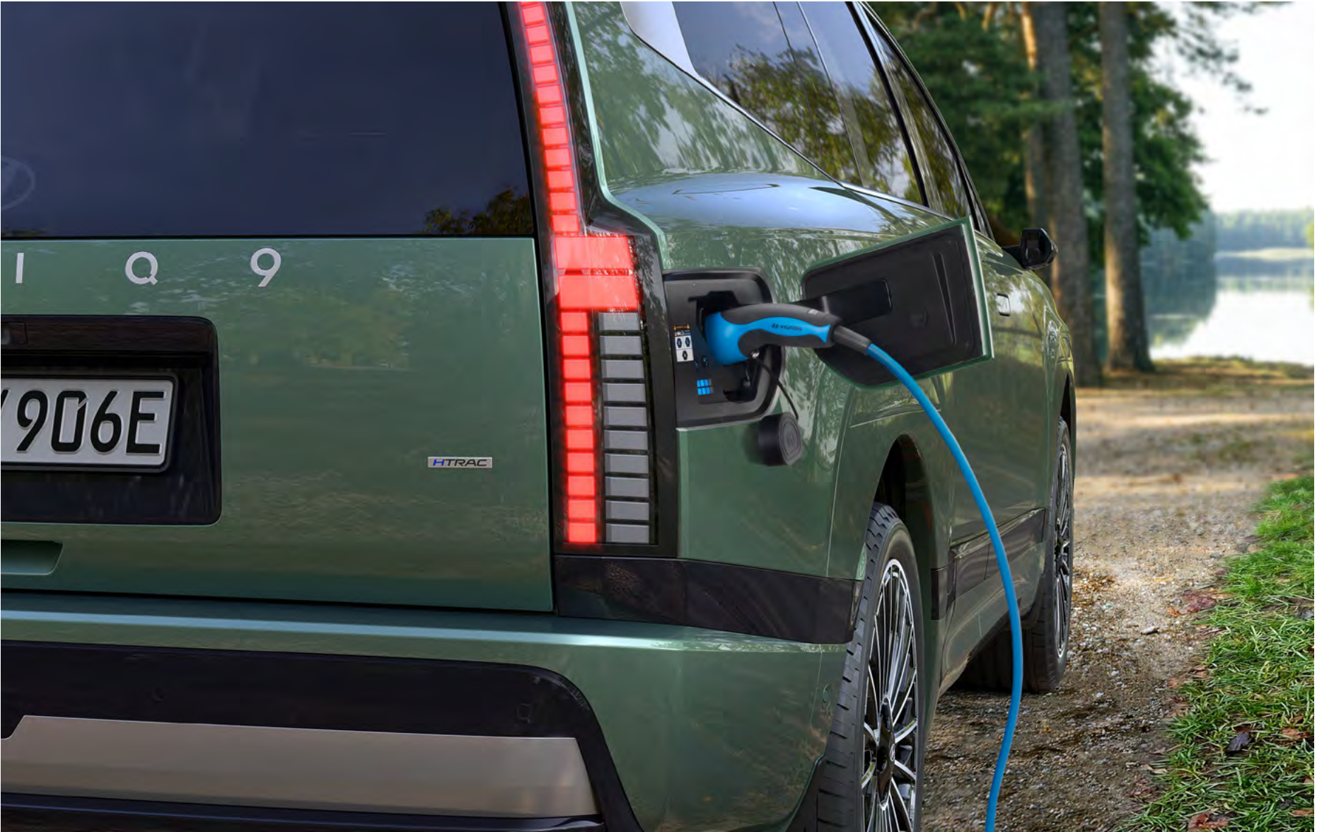
Charging cable, Mode 3 The Mode 3 charging cable is equipped with type-2 plugs at both ends and can be used for day-to-day charging at public and domestic charging points. 99632ADE003A (3-phase, 32 A, 5 m) 99632ADE003B (3-phase, 32 A, 7.5 m)
